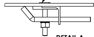
DETAIL A SCALE 1 : 4
