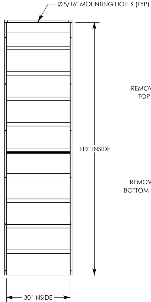
VIEW B-B
