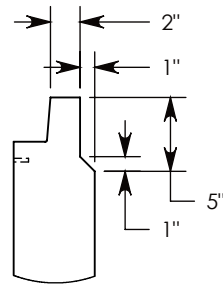
DETAIL B SCALE 1 : 13
