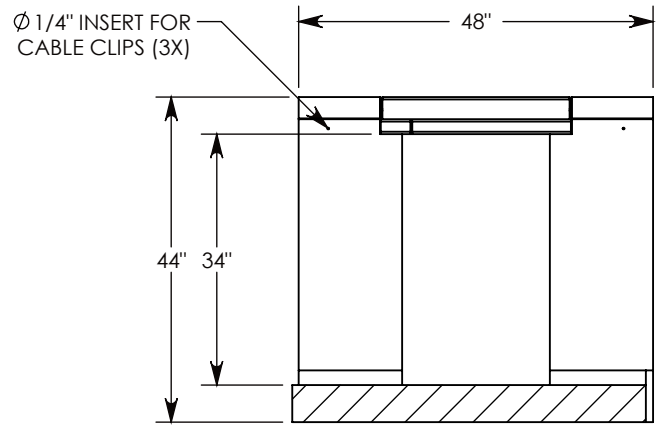
SECTION A-A AASHTO H-20 RATED - 32,000 LB. SINGLE AXLE LOAD
