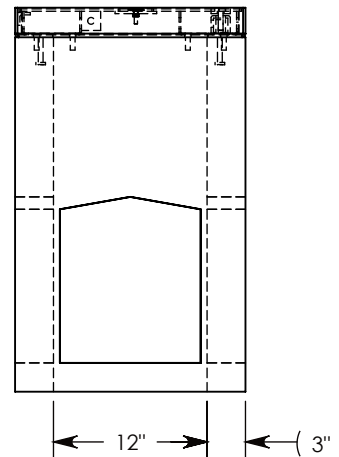
SIDE "C"
