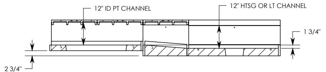
REF. SECTION VIEW OF TRANSITION CHANNEL ASSEMBLY
