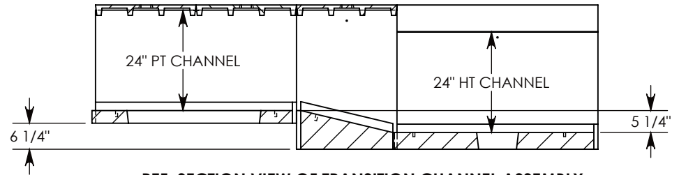
REF. SECTION VIEW OF TRANSITION CHANNEL ASSEMBLY
