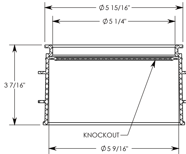
SECTION A-A SEAL RING HIDDEN
