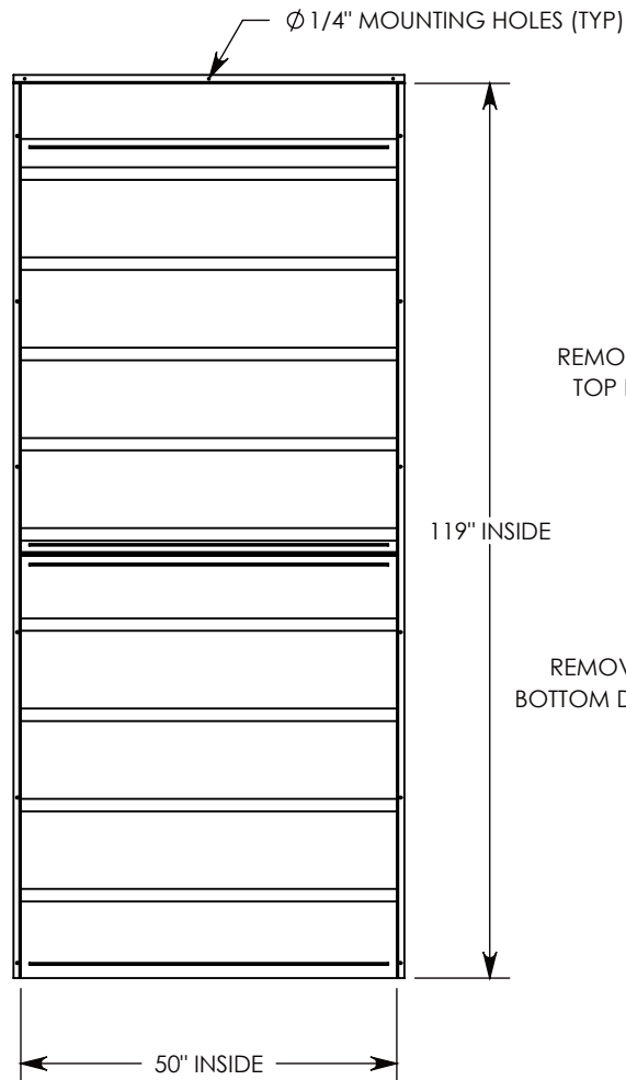
VIEW B-B
