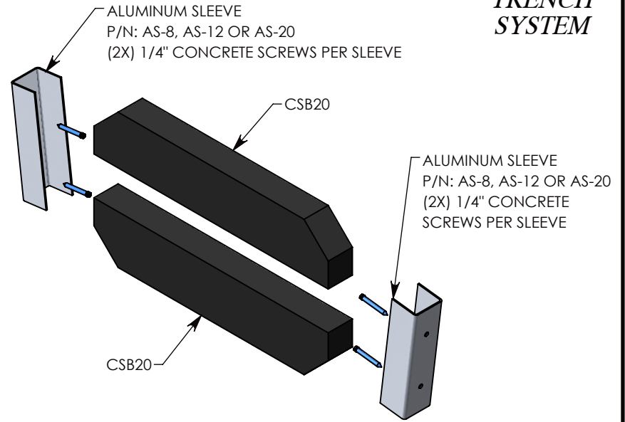
REFERENCE ASSEMBLY
