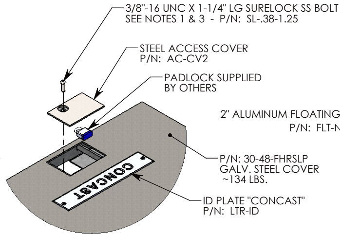
DETAIL A SCALE 1 : 11
